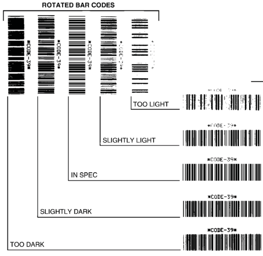
Figure 19 • Bar Code Darkness Comparison
