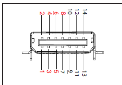
Figure 28: RS-232C Communications Port
